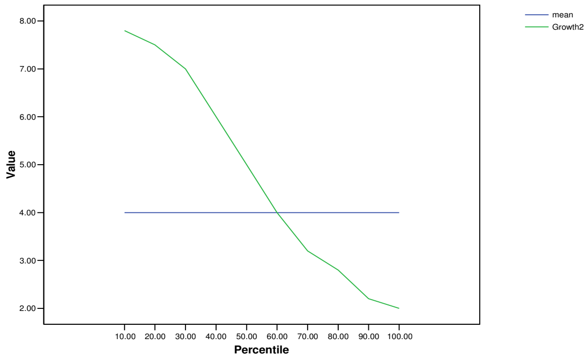
Figure 2: Growth Incidence Curve-Case 2
